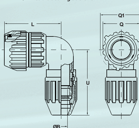
ITS-RRG (08) 90° Right-Angle Plug with EMI/RFI Cable Sealing Backshell
