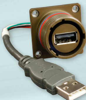
MIL-DTL-38999 Series III with USB jack and jumper
