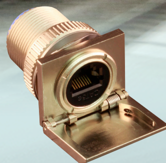
SuperSeal RJ45 connector with environmental flap-lid cover
