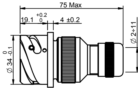
FRITS0020-RJ45-1PHMF6
