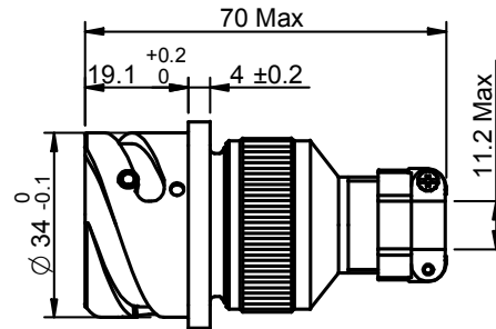
FRITS0020-RJ45-1N1F6
