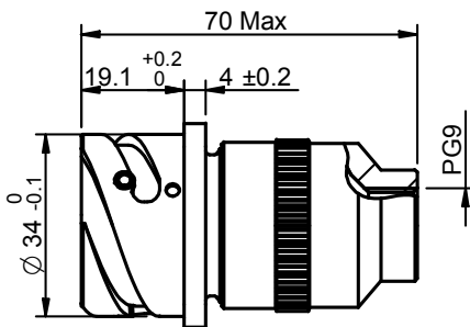
FRITS0020-RJ45-1PGF6
